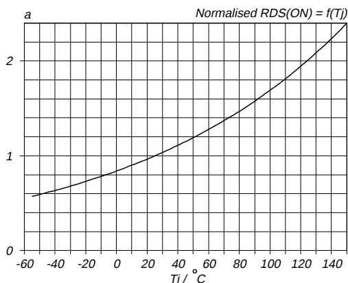
Fig. 9. Normalised drain-source on-state resistance. a = R_{DS(ON)}/R_{DS(ON)25^\circ\text{C}} = f(T_j) ; I_D = 1.7\text{ A} ; V_{GS} = 10\text{ V}
