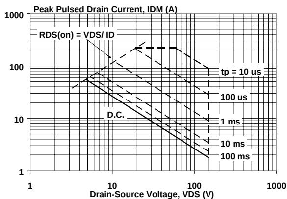
Fig.3. Safe operating area. T_{mb} = 25^\circ\text{C} I_D \text{ \& } I_{DM} = f(V_{DS}); I_{DM} \text{ single pulse; parameter } t_p
