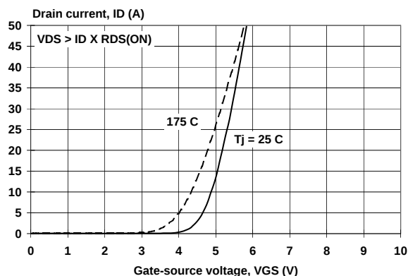
Fig.7. Typical transfer characteristics. I_D = f(V_{GS}) ; parameter T_j
