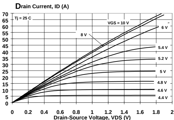
Fig.5. Typical output characteristics, T_j = 25^\circ\text{C} . I_D = f(V_{DS}); \text{ parameter } V_{GS}
