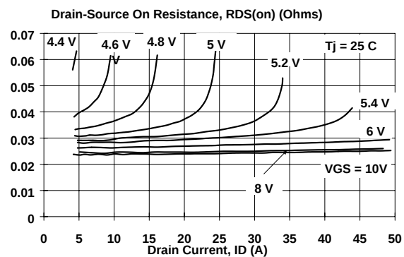
Fig.6. Typical on-state resistance, T_j = 25^\circ\text{C} . R_{DS(ON)} = f(V_{GS})
