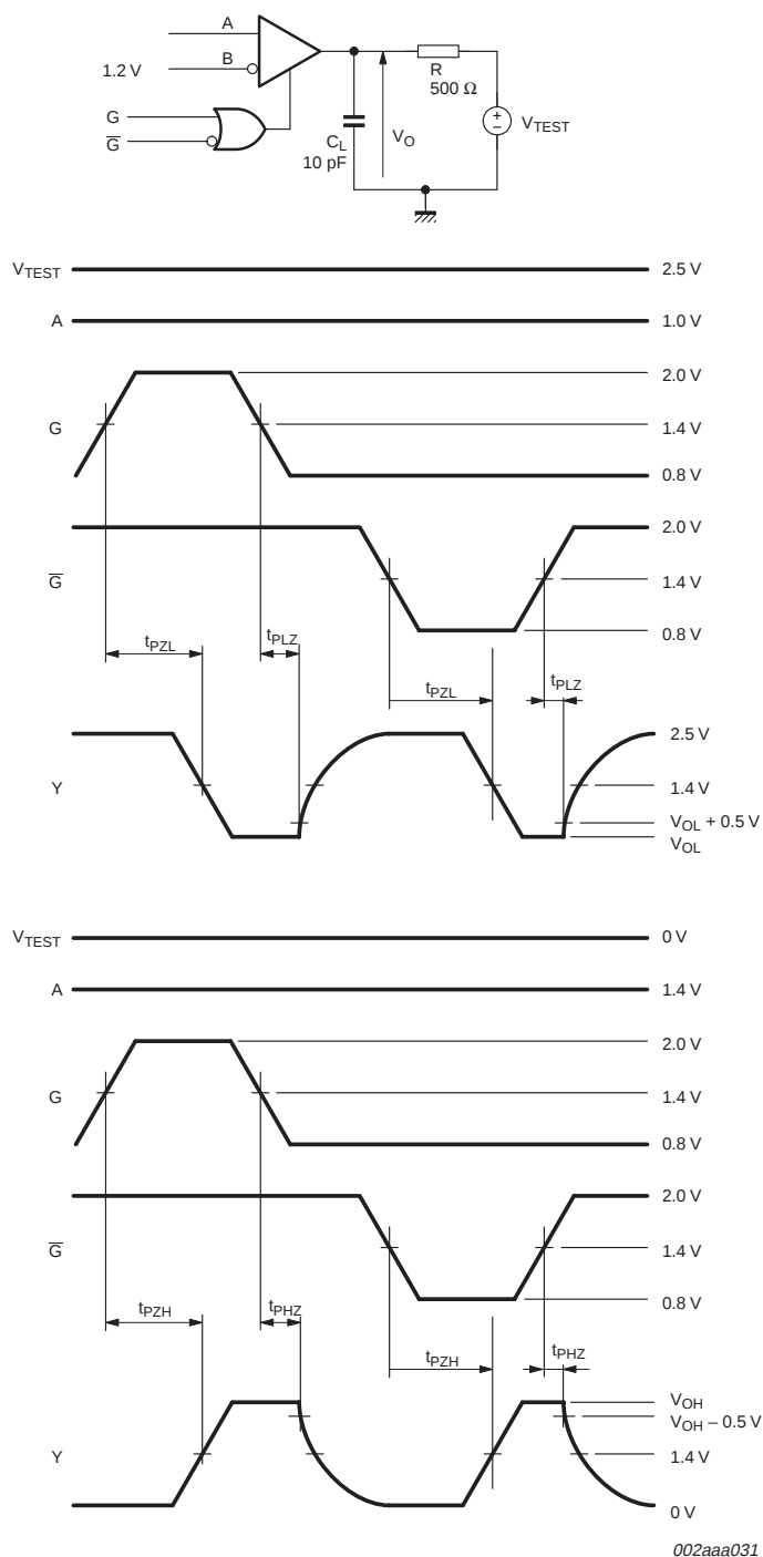
Fig 6. Enable/disable time test circuit and waveforms.
