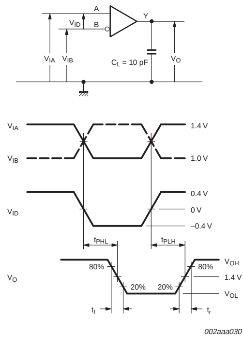
Fig 5. Timing test circuit and waveforms.
