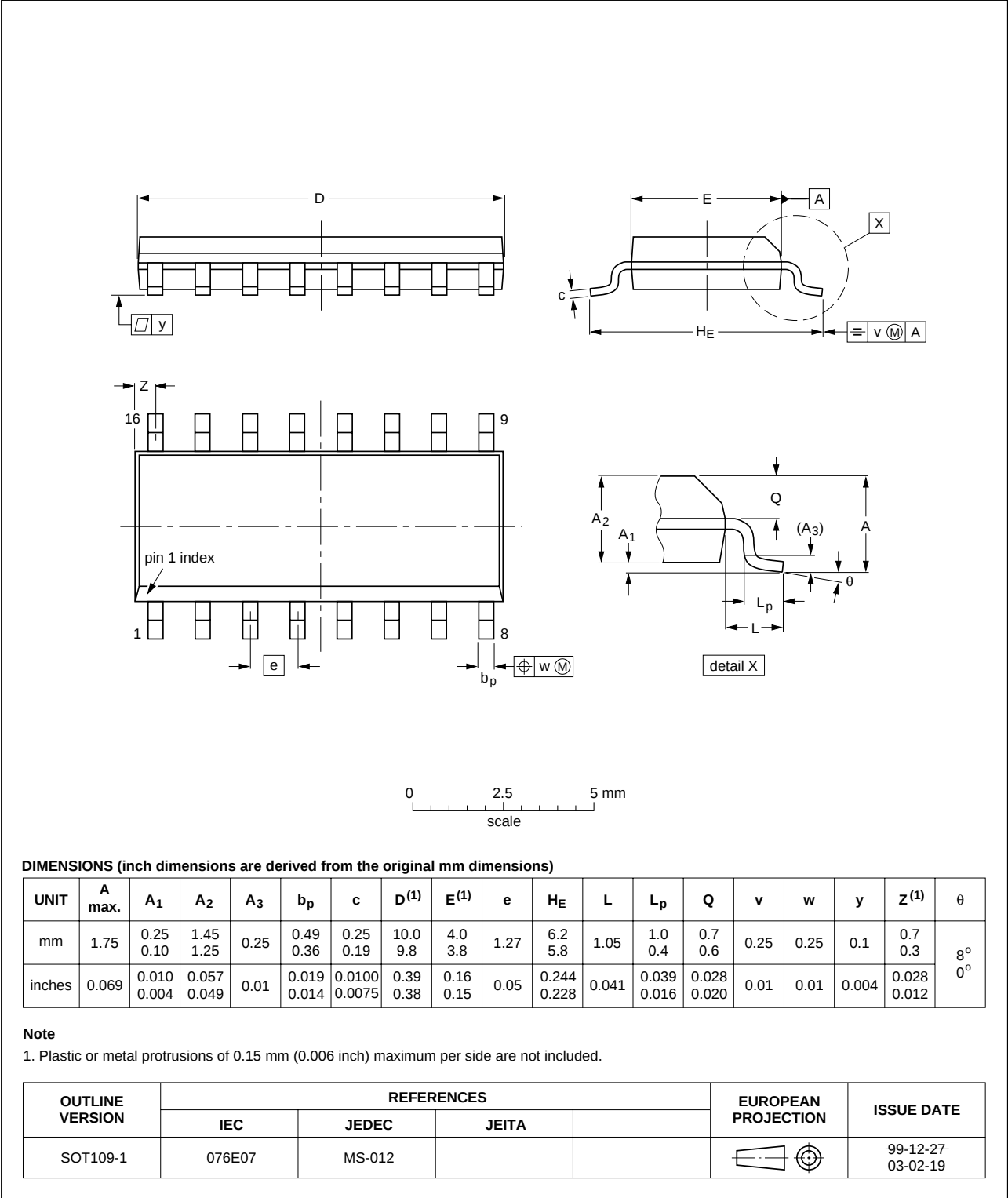
Fig 8. SO16 package outline (SOT109-1).
