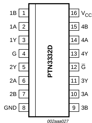
Fig 2. SO16 pin configuration.
