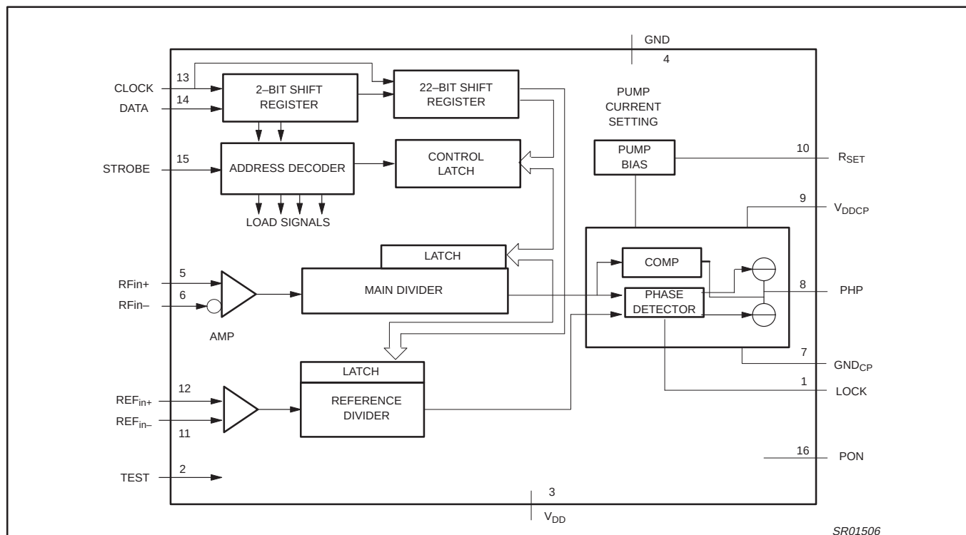
Figure 2. Block Diagram
