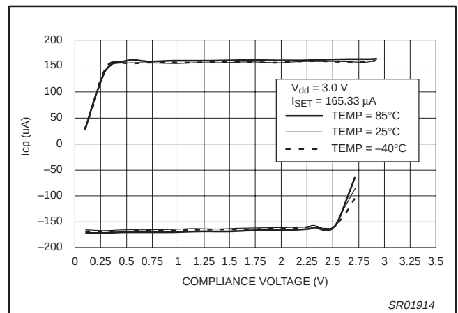
Figure 12. Php Charge Pump Output vs. Temperature (CP = 1; V_{DD} = 3.0 V; I_{SET} = 165.33 \mu A)
