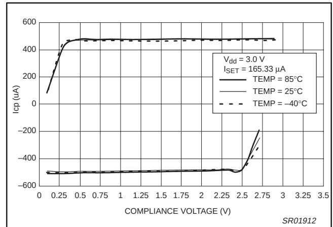
Figure 10. Php Charge Pump Output vs. Temperature (CP = 0; V_{DD} = 3.0 V; I_{SET} = 165.33 \mu A)
