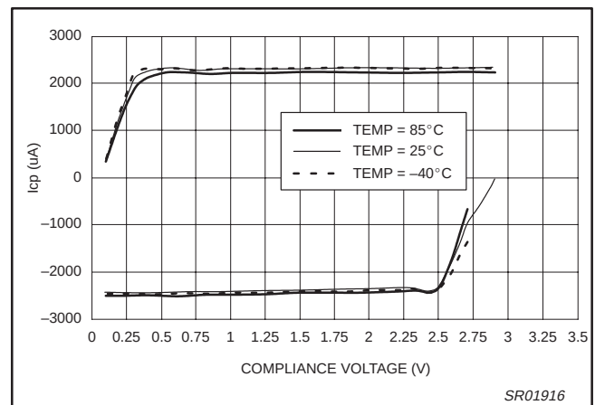
Figure 14. Php-su Charge Pump Output vs. Temperature (CP = 0; V_{DD} = 3.0 V; I_{SET} = 165.33 \mu A)
