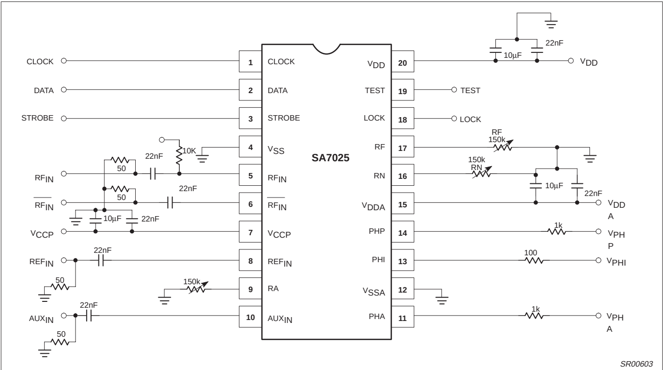
Figure 4. Test Circuit
