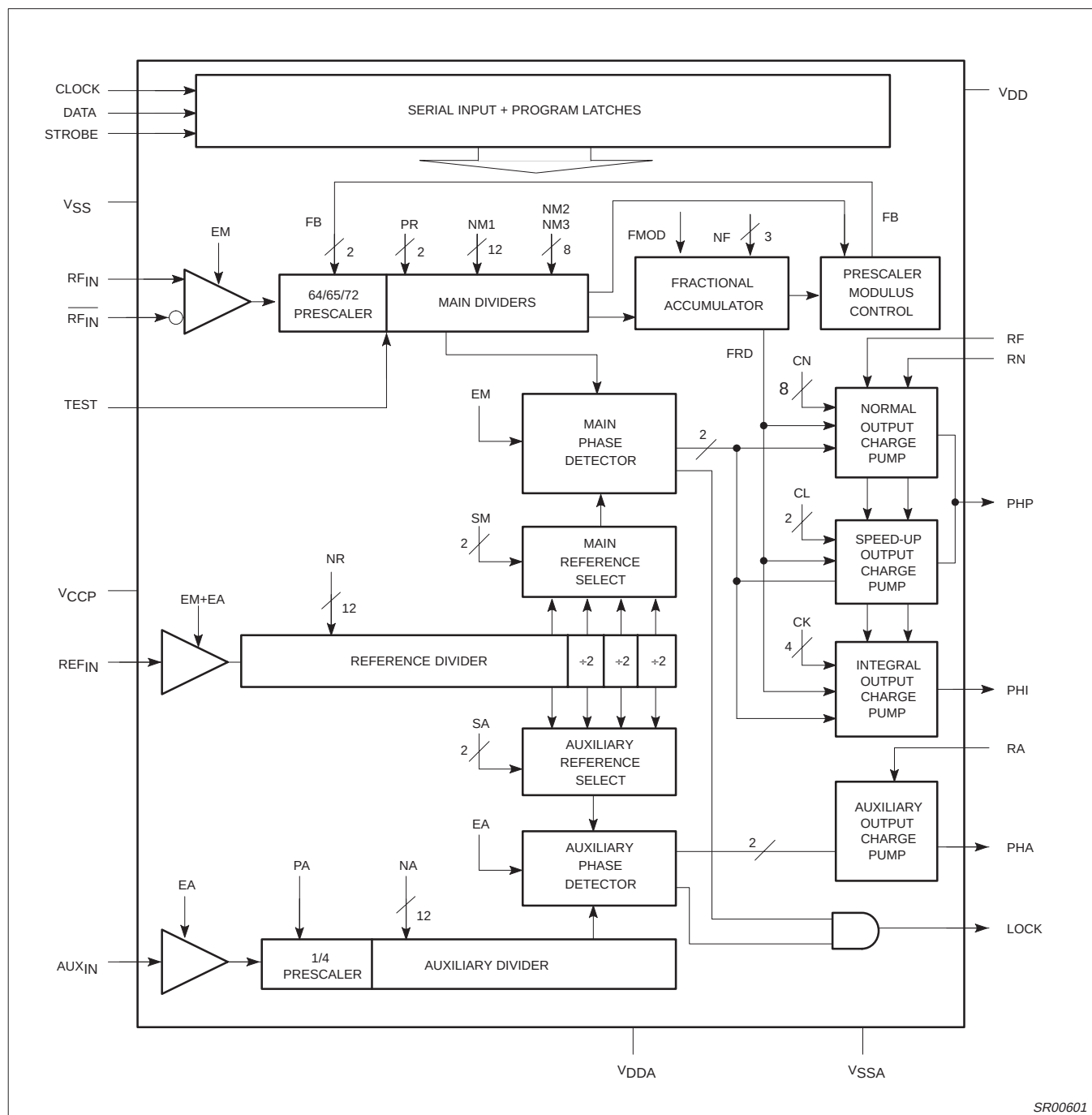
Figure 2. Block Diagram
