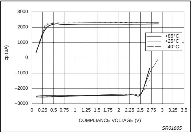
Figure 20. PHP-SU Charge Pump Output vs. Temperature (CP = 00; V_{DD} = 3.0 V; I_{SET} = 165.33 \mu A)
