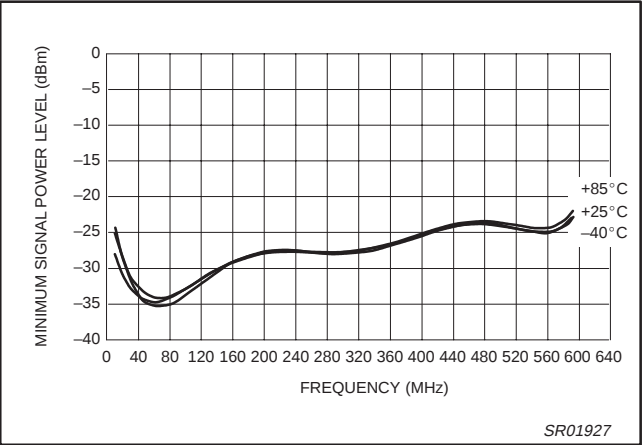
Figure 28. Auxiliary Divider Input Sensitivity vs. Frequency and Temperature (VDD = 3.00 V)
