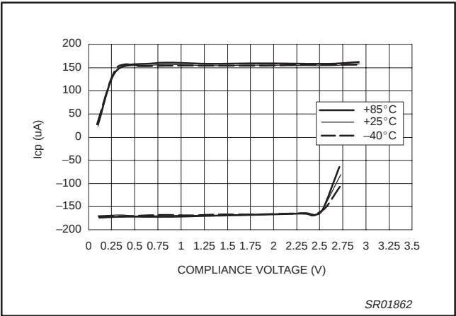
Figure 16. PHP Charge Pump Output vs. Temperature (CP = 11; V_{DD} = 3.0 V; I_{SET} = 165.33 \mu A)
