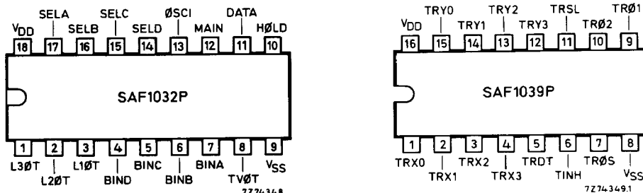
Fig. 1 Pin designations.
