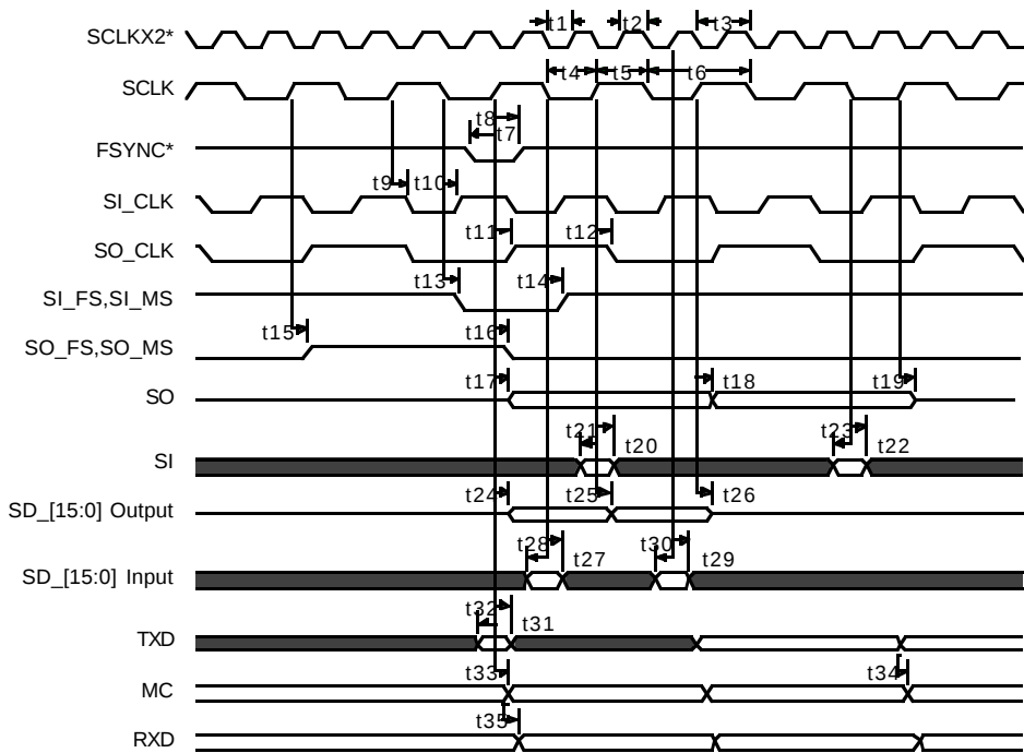
Figure 4. Local Bus Interface Timing — SCbus Mode (4.096 Mbps)
