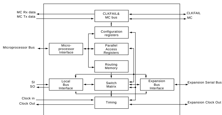
Block Diagram
