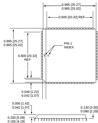
Package Mechanical Drawing
