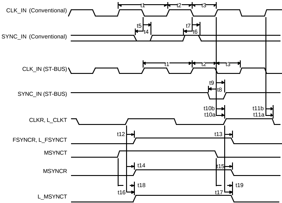
Figure 13. CLK_IN, SYNC_IN — PEB Network Master Mode (CLK_IN Divider ≥ 2)
