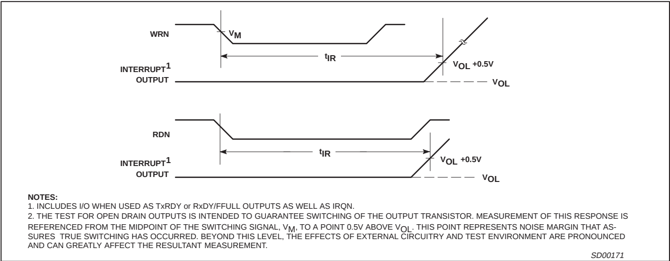
Figure 13. Interrupt Timing
