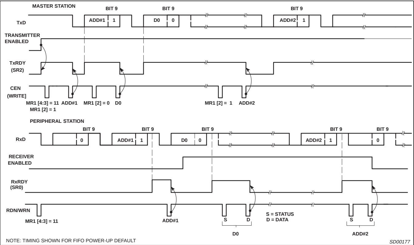
Figure 19. Wake-Up Mode
