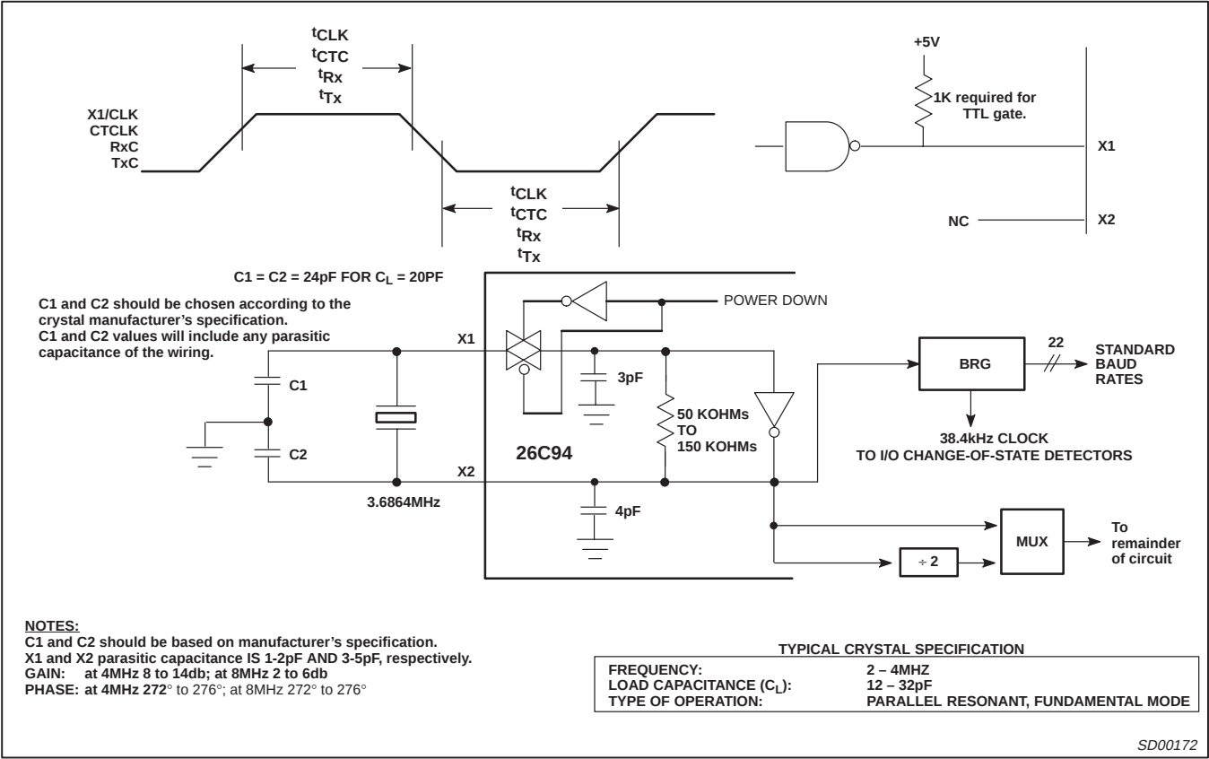
Figure 14. Clock Timing
