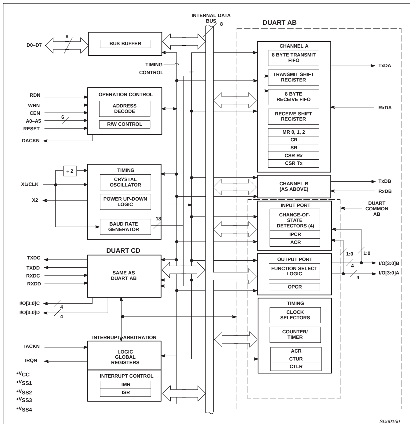
Figure 3. Block Diagram
