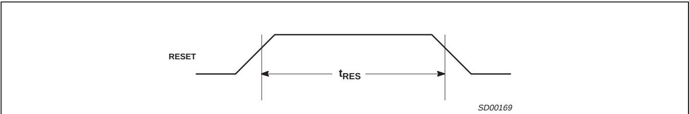
Figure 11. Reset Timing
