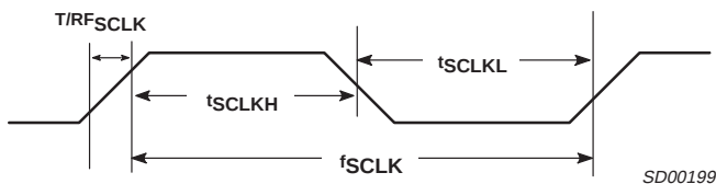
Figure 10. SCLK Timing
