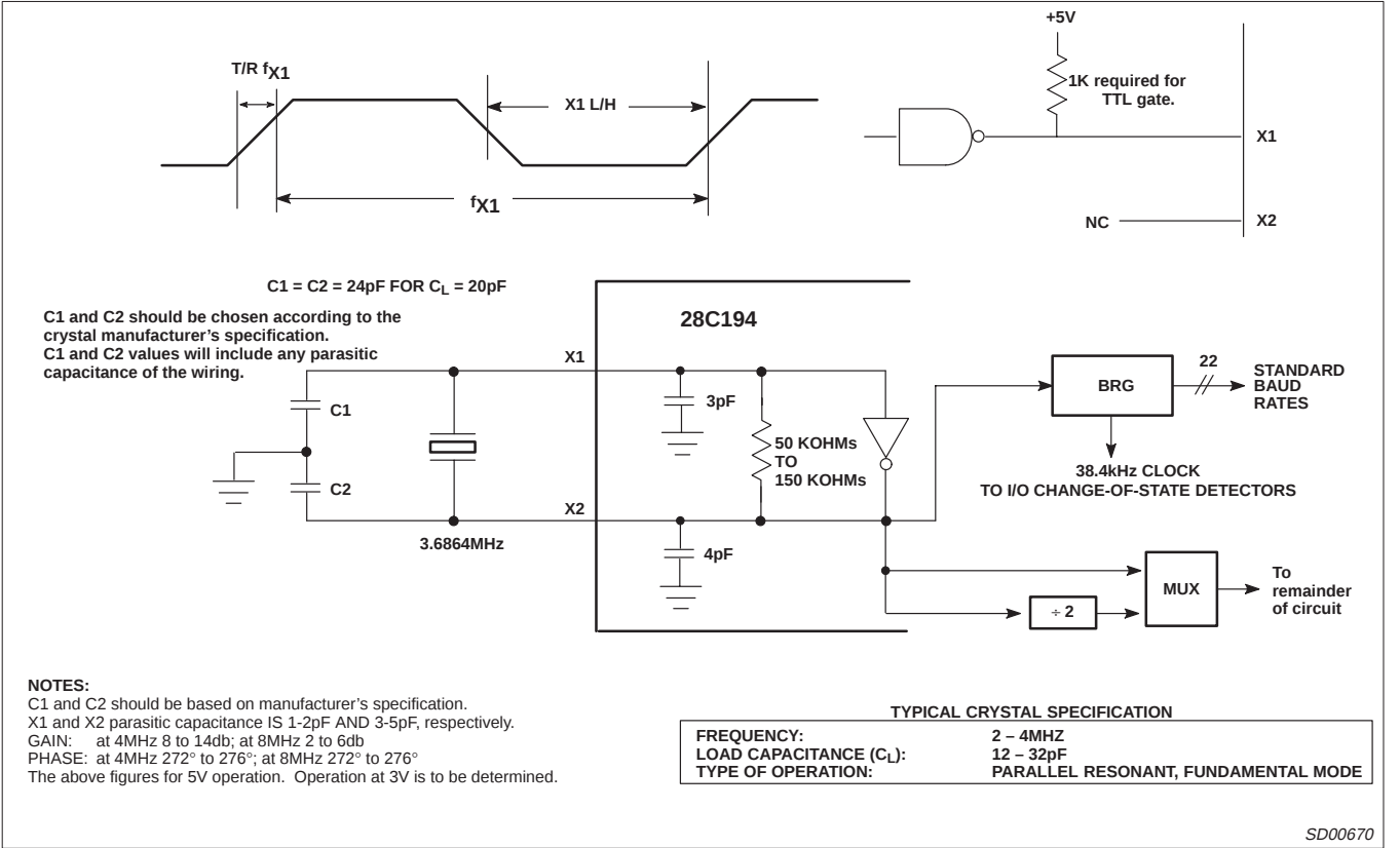
Figure 9. X1/X2 Communication Crystal Clock
