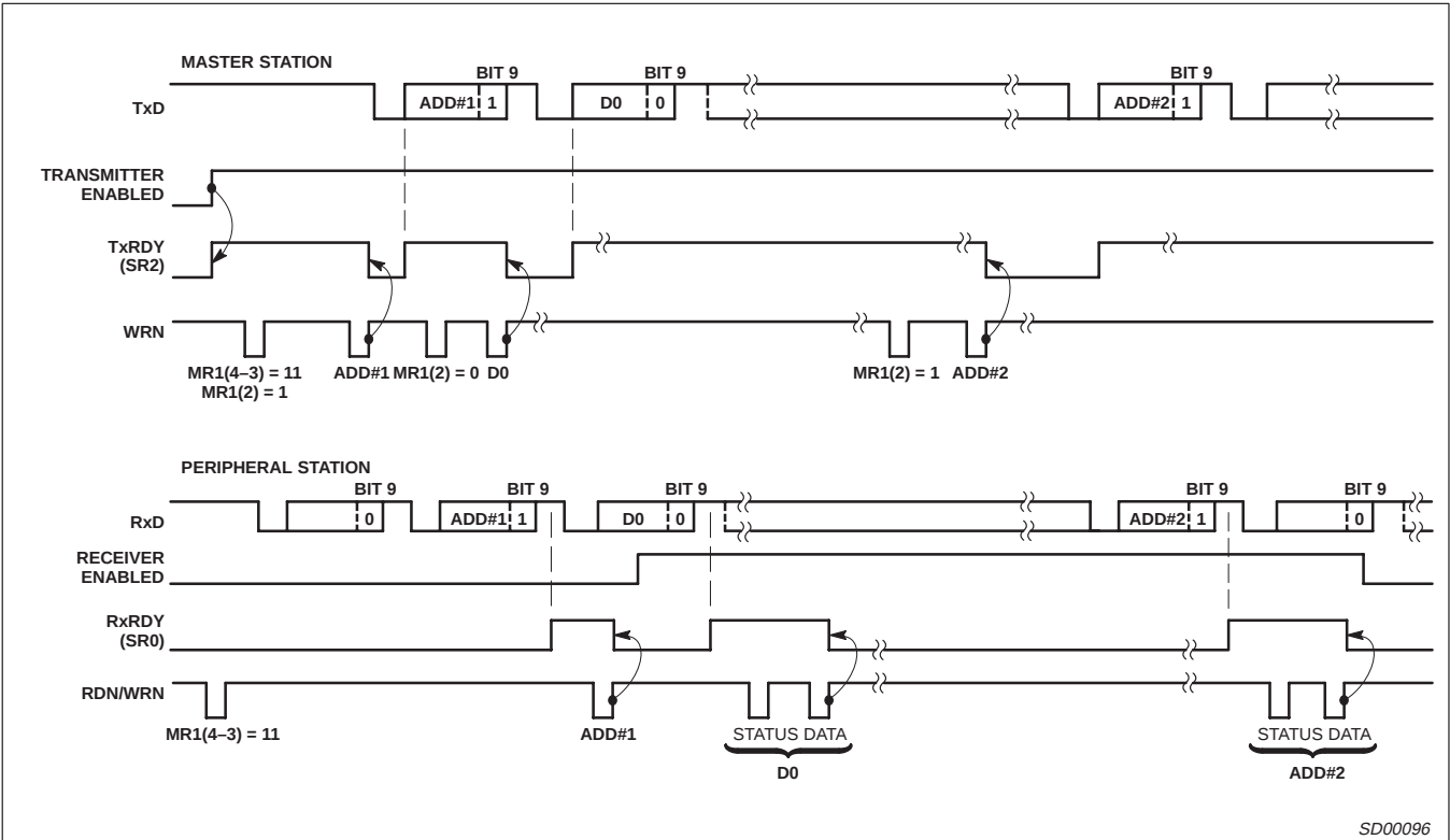
Figure 16. Wake-Up Mode
