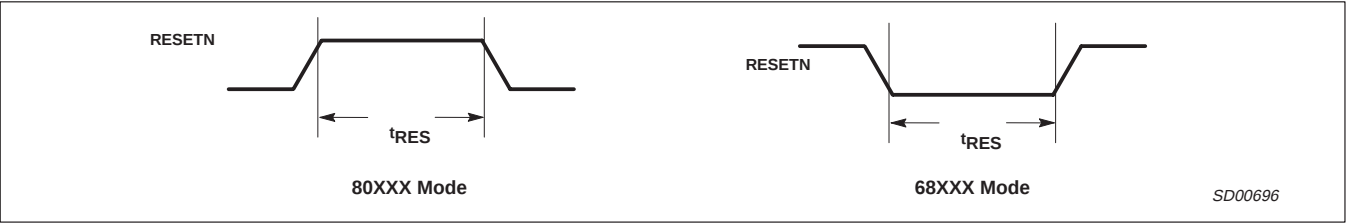
Figure 4. Reset Timing
