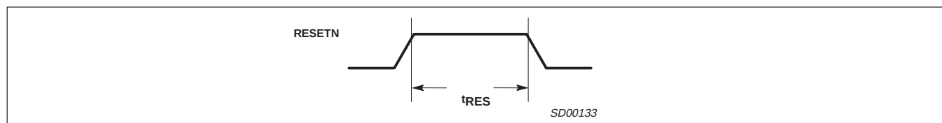
Figure 3. Reset Timing
