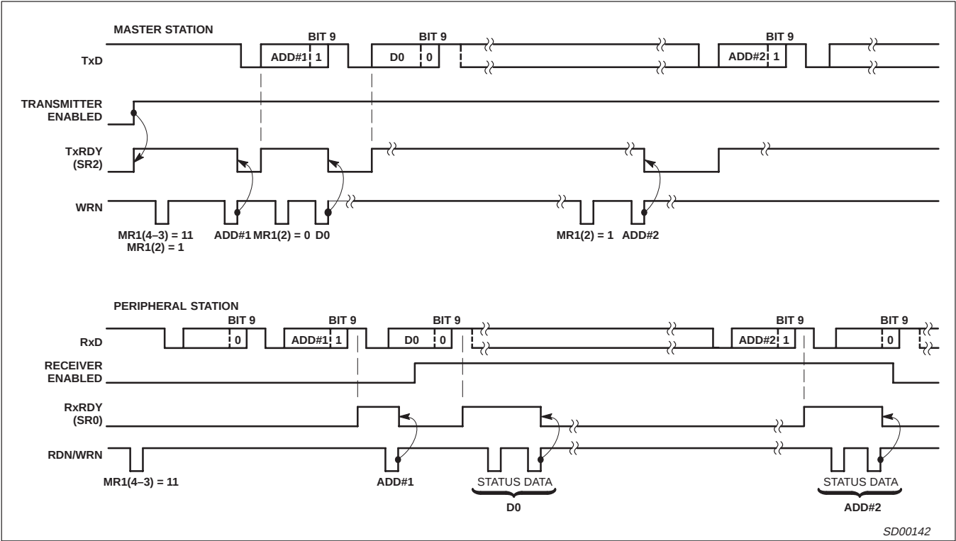
Figure 12. Wake-Up Mode
