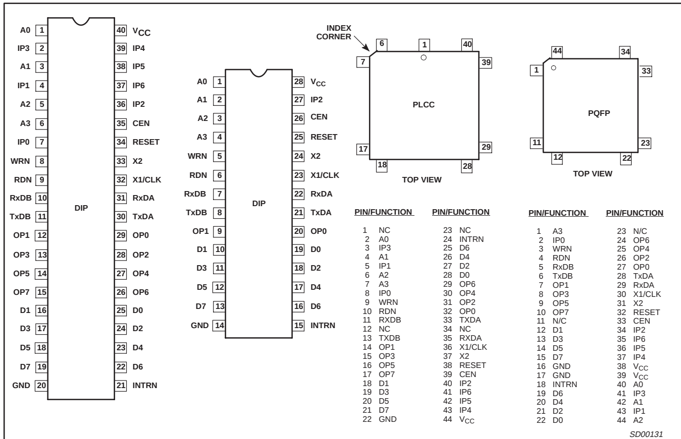
Figure 1. Pin Configurations
