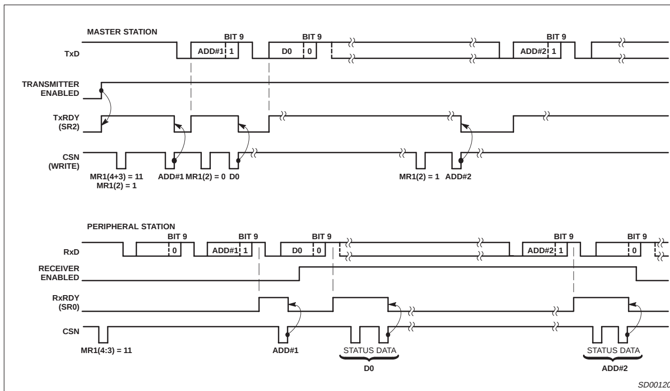
Figure 14. Wake-Up Mode
