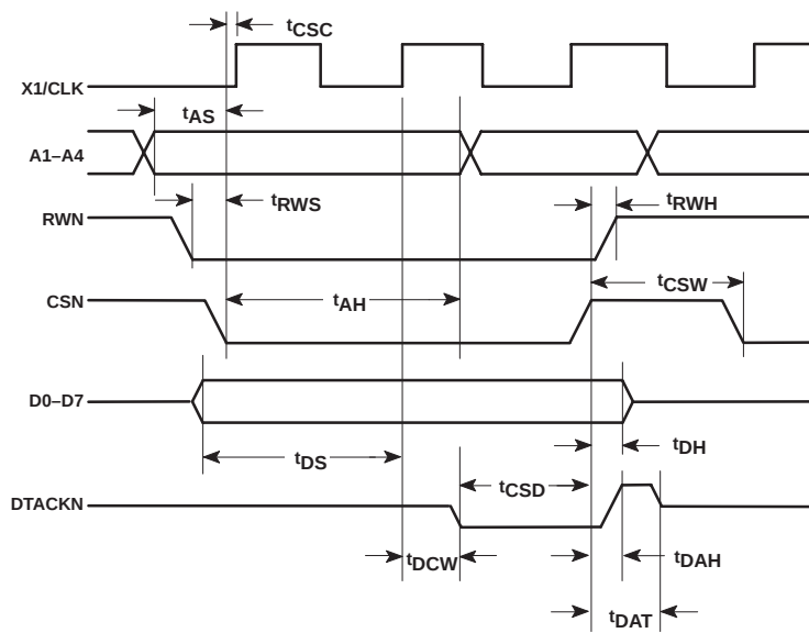
Figure 5. Bus Timing (Write Cycle)
