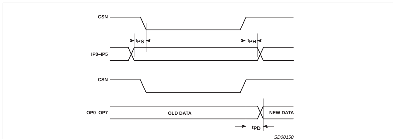
Figure 7. Port Timing
