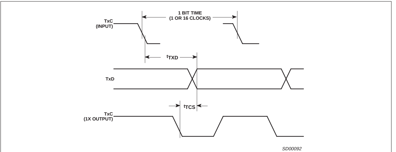
Figure 8. Transmit
