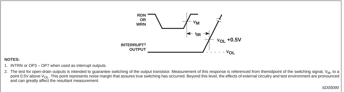
Figure 6. Interrupt Timing
