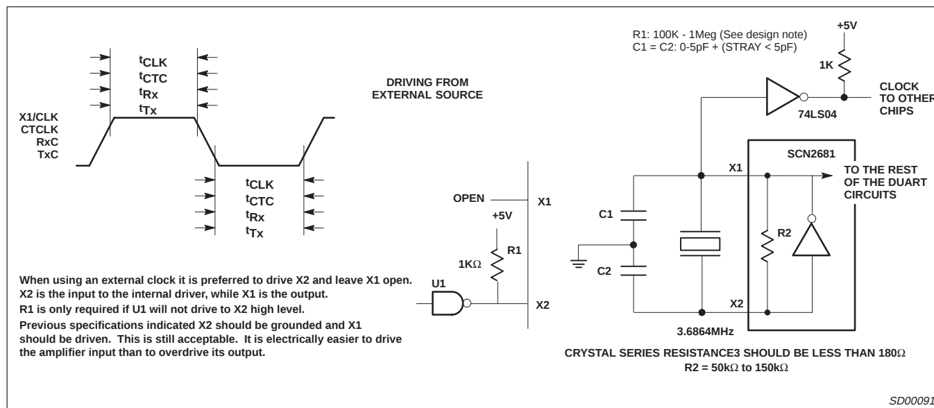
Figure 7. Clock Timing
