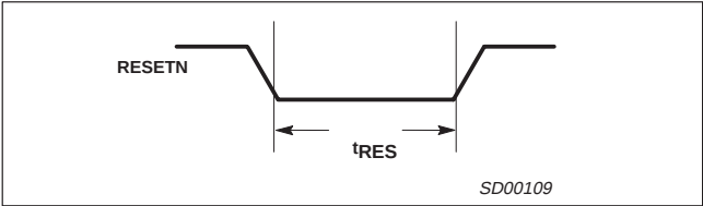
Figure 3. Reset Timing
