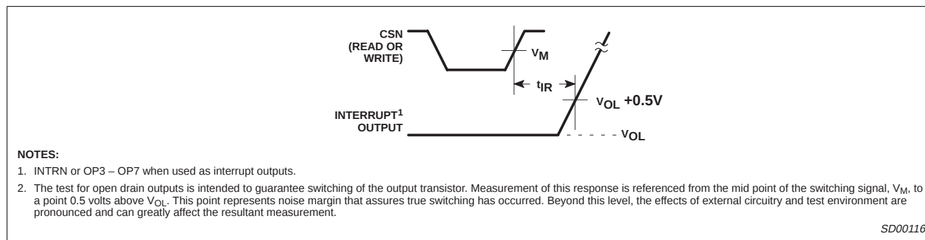
Figure 10. Interrupt Timing
