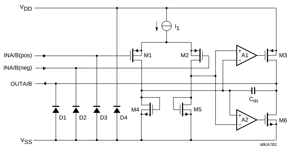
Fig.3 Equivalent schematic diagram.
