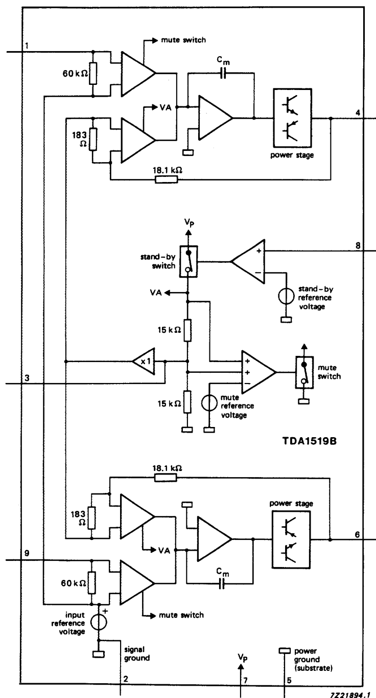
Fig.1 Block diagram.
