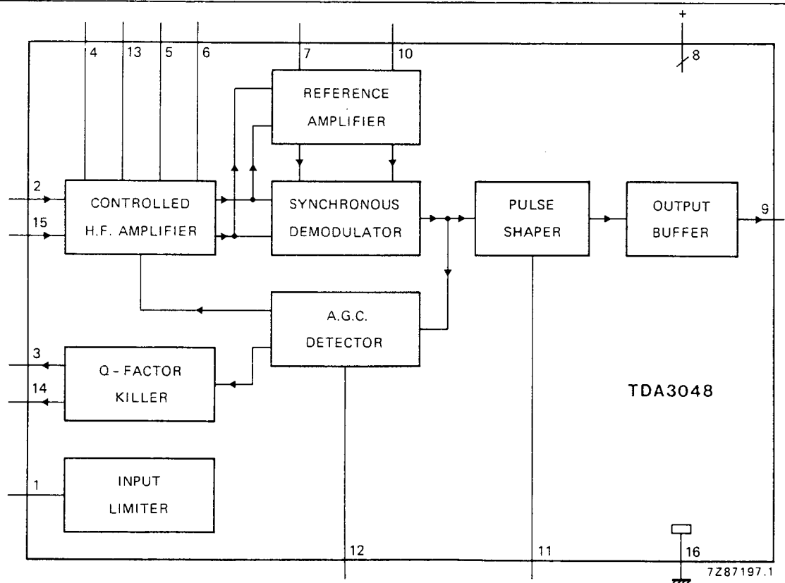
Fig. 1 Block diagram of TDA3048.
