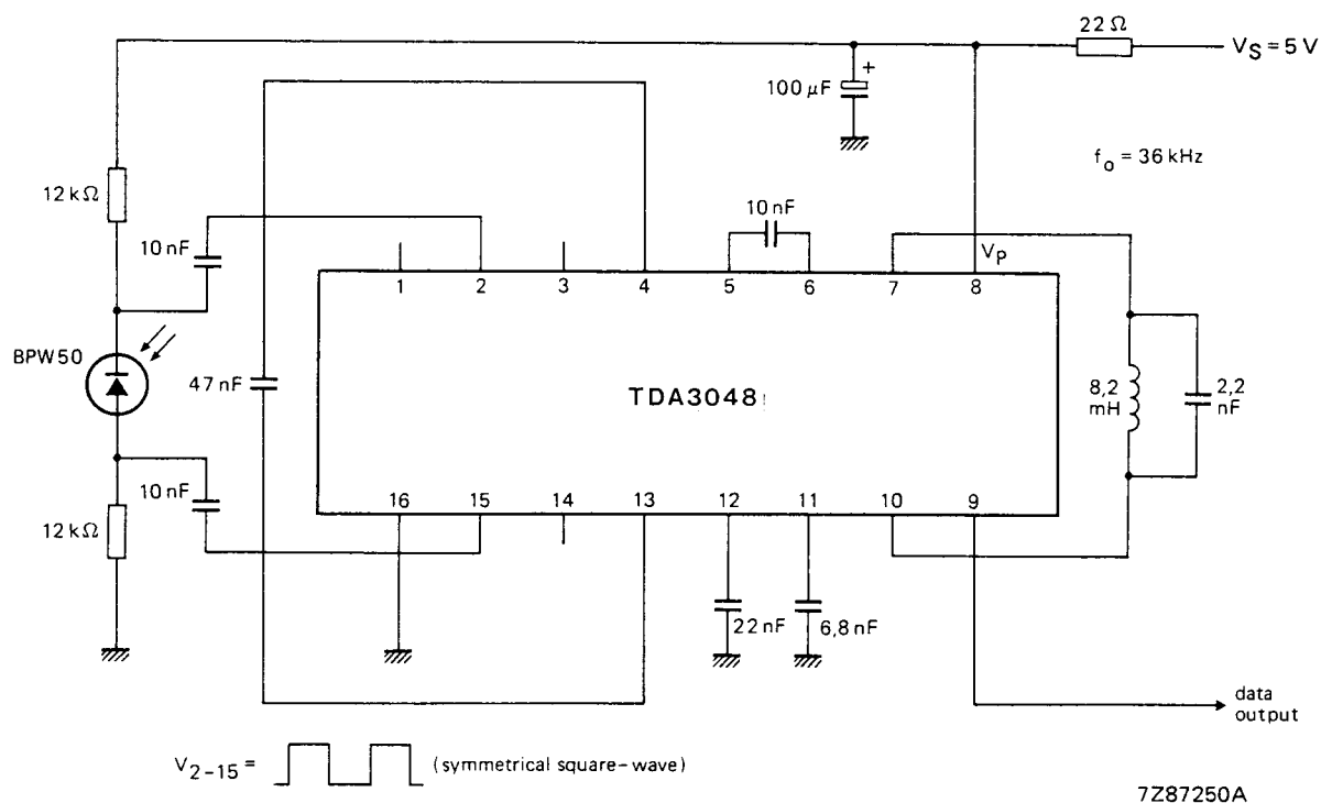
Fig. 4 Wide-band receiver with TDA3048.
