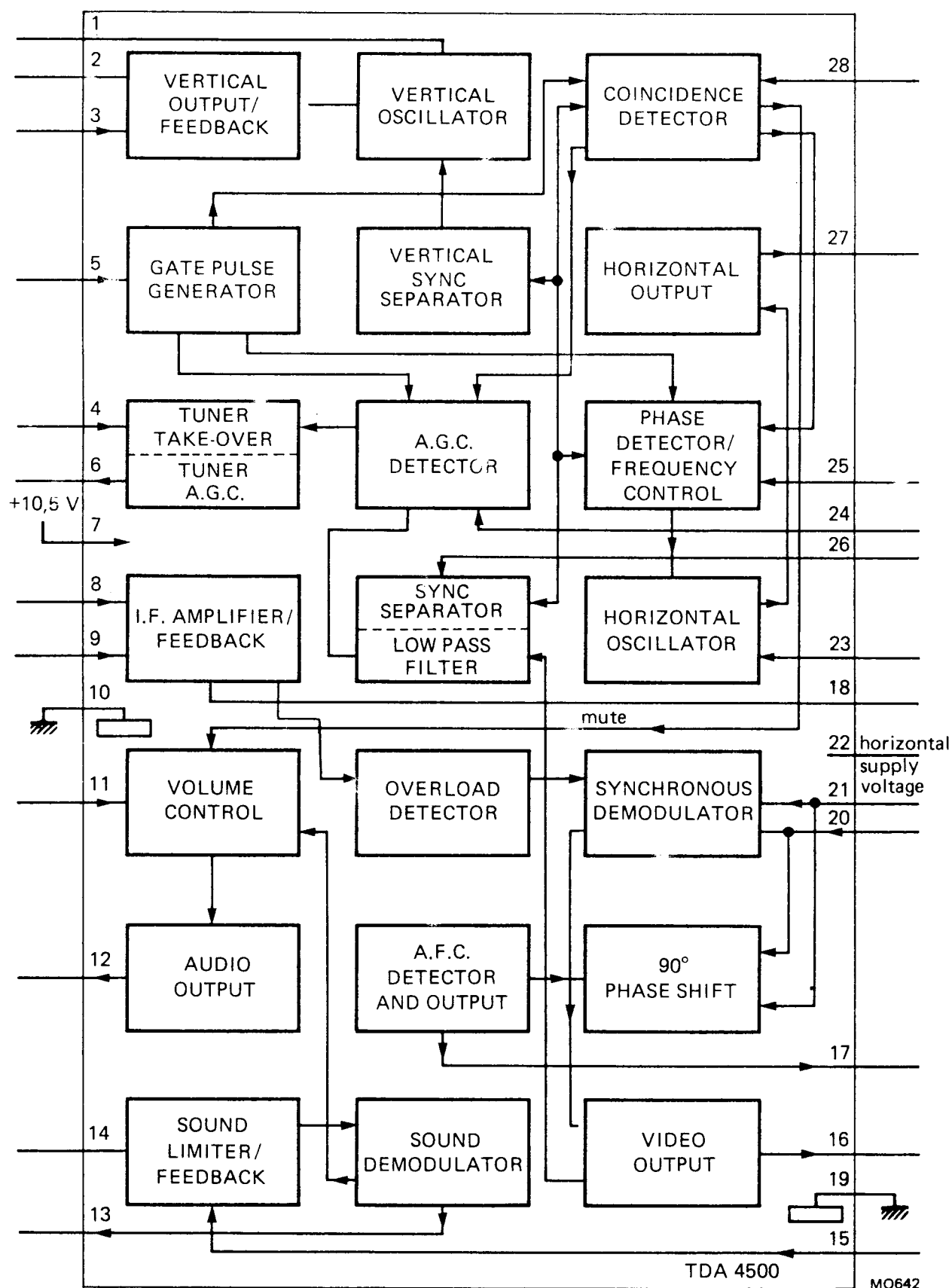
Fig. 1 Block diagram.
