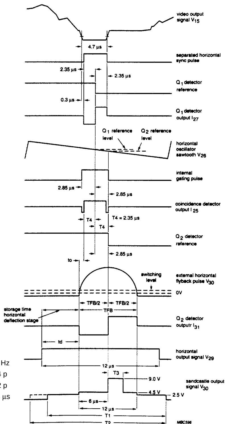
Fig.6 Timing diagram.
