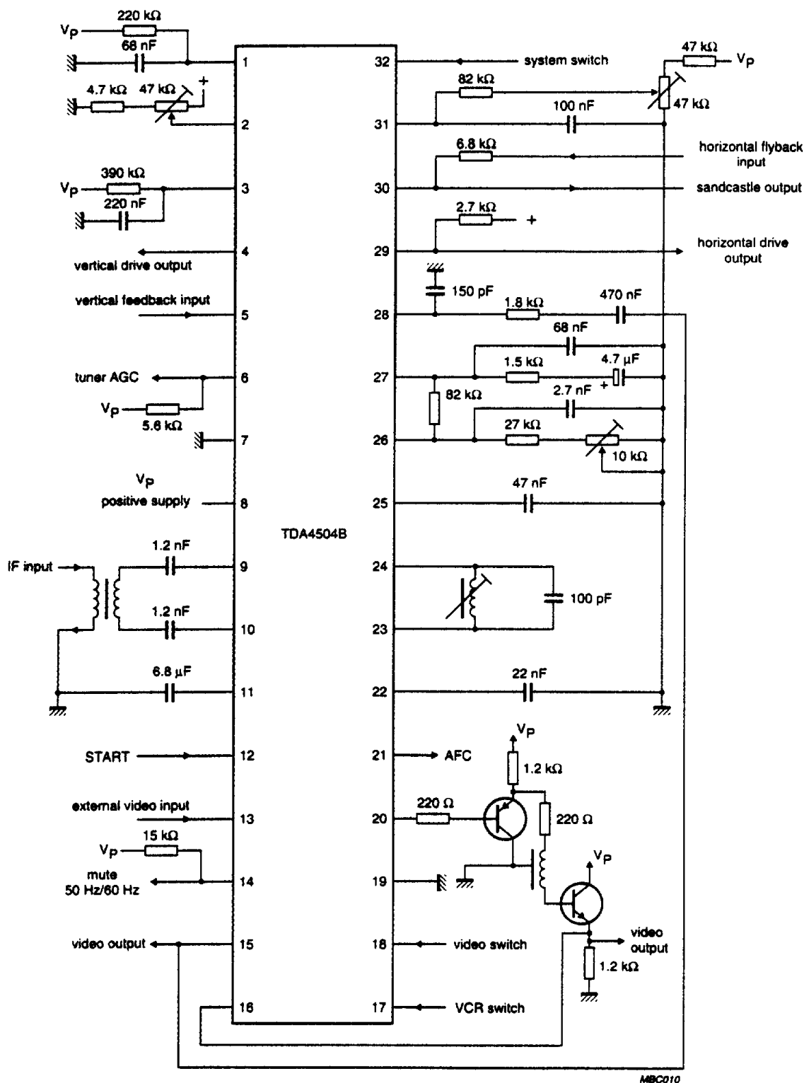
Fig.9 Application diagram.
