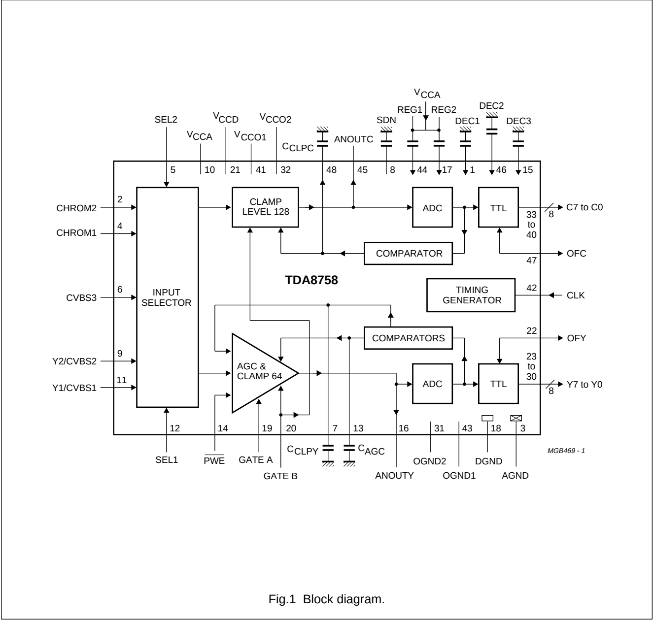
BLOCK DIAGRAM
