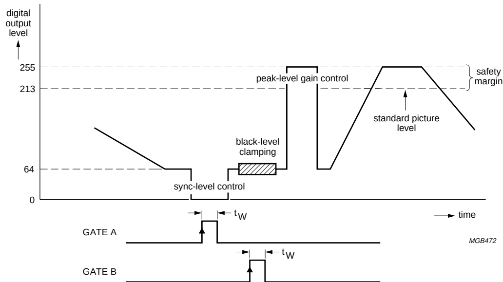
Fig.6 Control mode Y channel.
