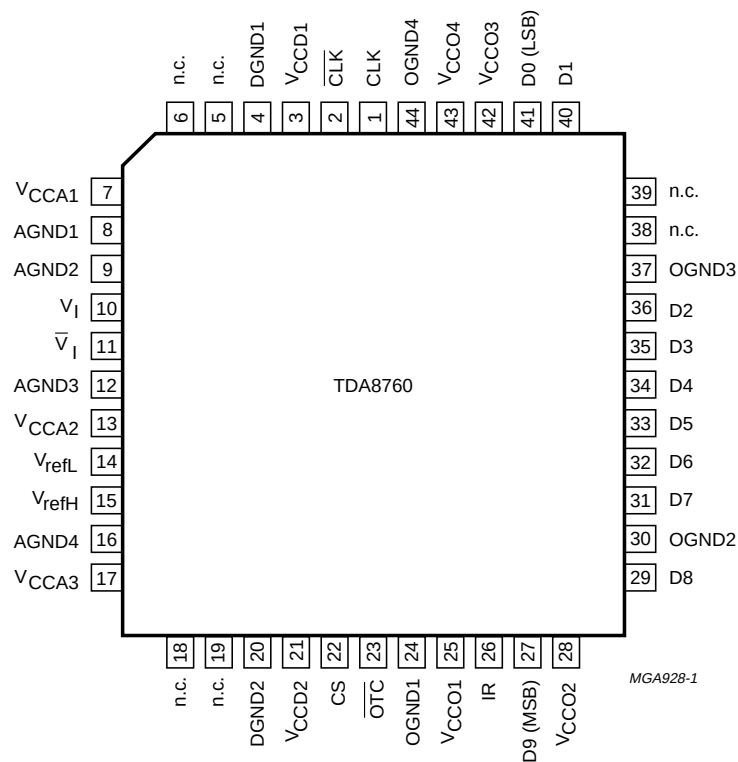
Fig.2 Pin configuration for SOT187-2.
