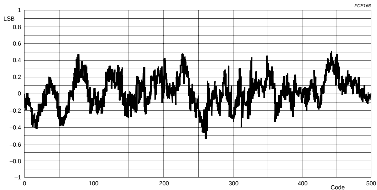
Fig.9 Typical AC INL ( f_{\text{clk}} = 30 \text{ MHz} ; f_i = 10 \text{ MHz} ).
