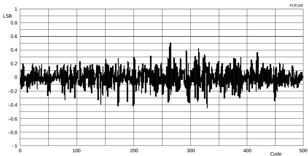
Fig.10 Typical AC DNL ( f_{\text{clk}} = 30 \text{ MHz} ; f_i = 10 \text{ MHz} ).
