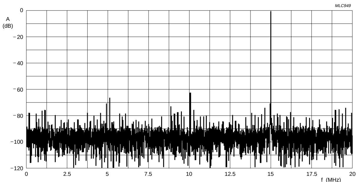
Fig.9 Fast Fourier Transform ( f_{\text{clk}} = 40 \text{ MHz} ; f_i = 15 \text{ MHz} ).
