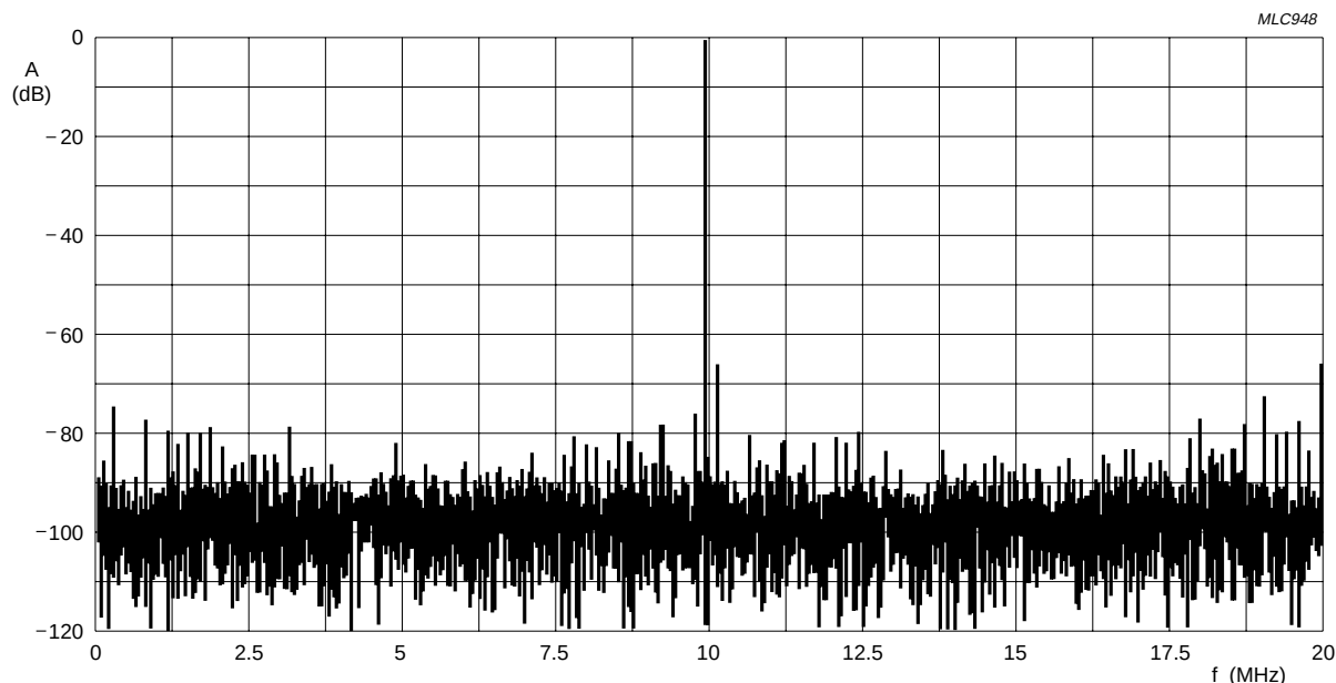
Fig.8 Fast Fourier Transform ( f_{\text{clk}} = 40 \text{ MHz} ; f_i = 10 \text{ MHz} ).
