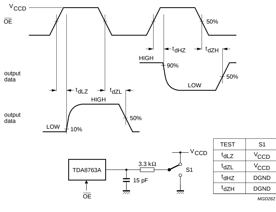
Fig.5 Timing diagram and test conditions of 3-state output delay time.
