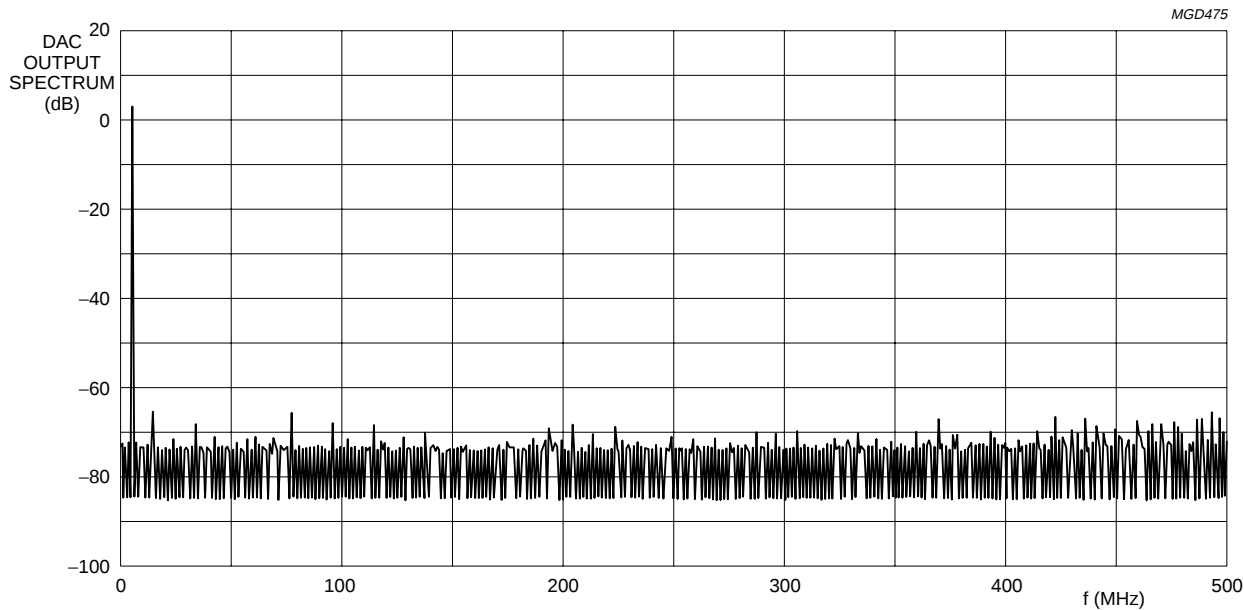
Fig.4 Typical output spectrum; f_{clk} = 1000\text{ MHz} ; f_{OUT} = 10\text{ MHz} .
