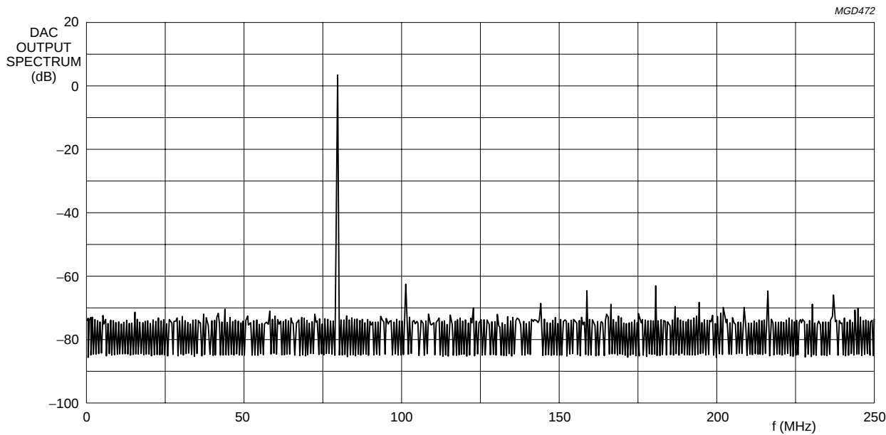
Fig.6 Typical output spectrum; f_{clk} = 500\text{ MHz} ; f_{OUT} = 80\text{ MHz} .
