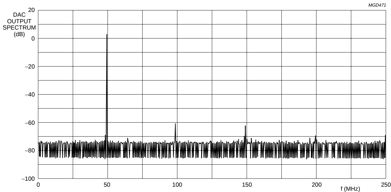
Fig.5 Typical output spectrum; f_{clk} = 500\text{ MHz} ; f_{OUT} = 50\text{ MHz} .
