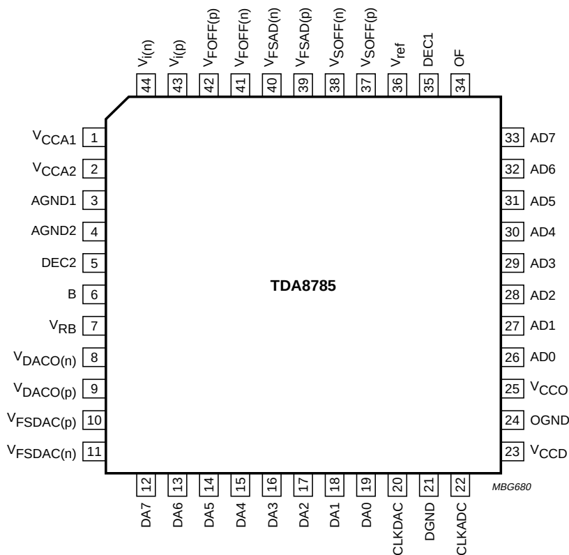
Fig.2 Pin configuration.
