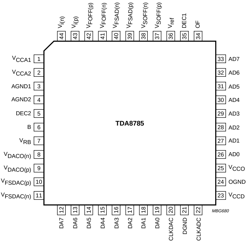
Fig.2 Pin configuration.
