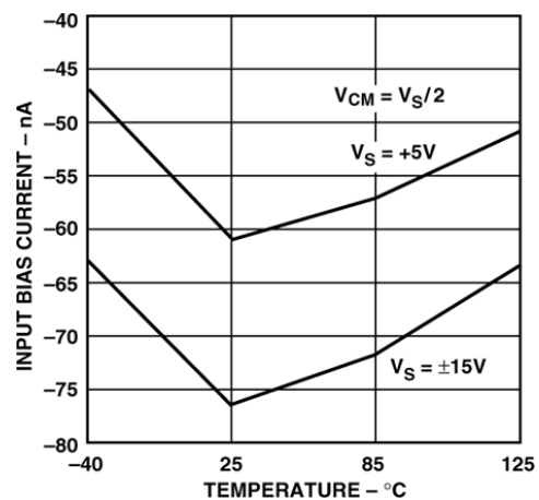
FIGURE 6. BIAS CURRENT VS. TEMPERATURE
