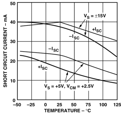
FIGURE 11. SHORT CIRCUIT CURRENT VS. TEMPERATURE
