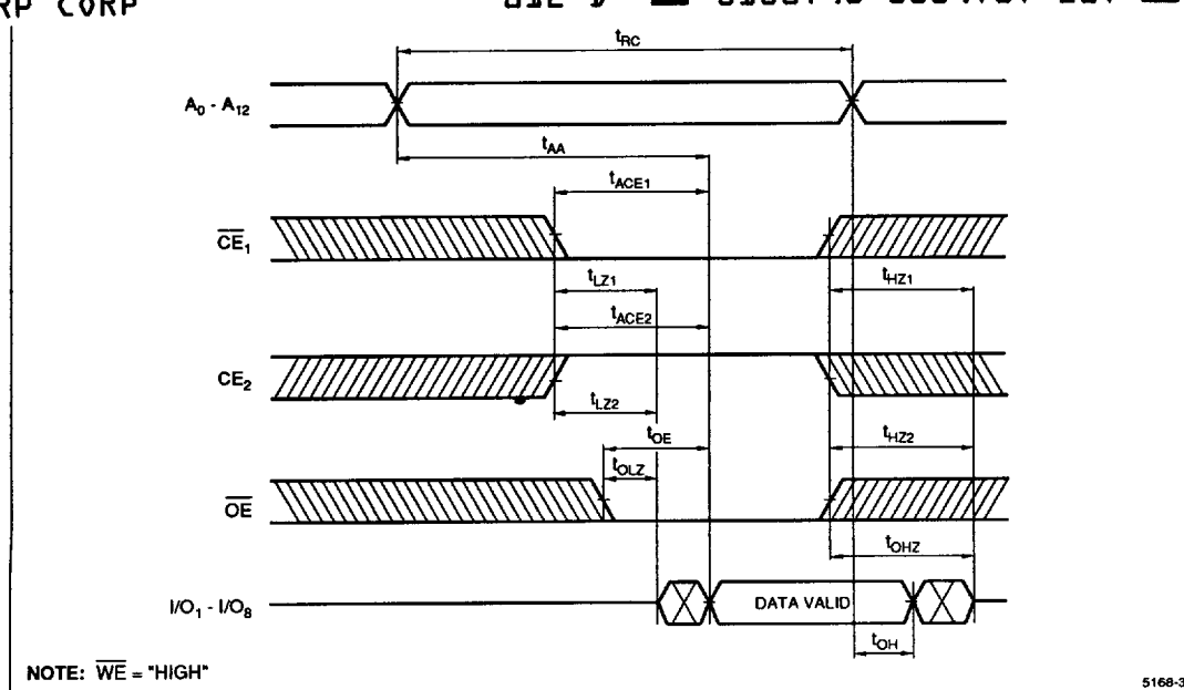
Figure 5. Read Cycle
