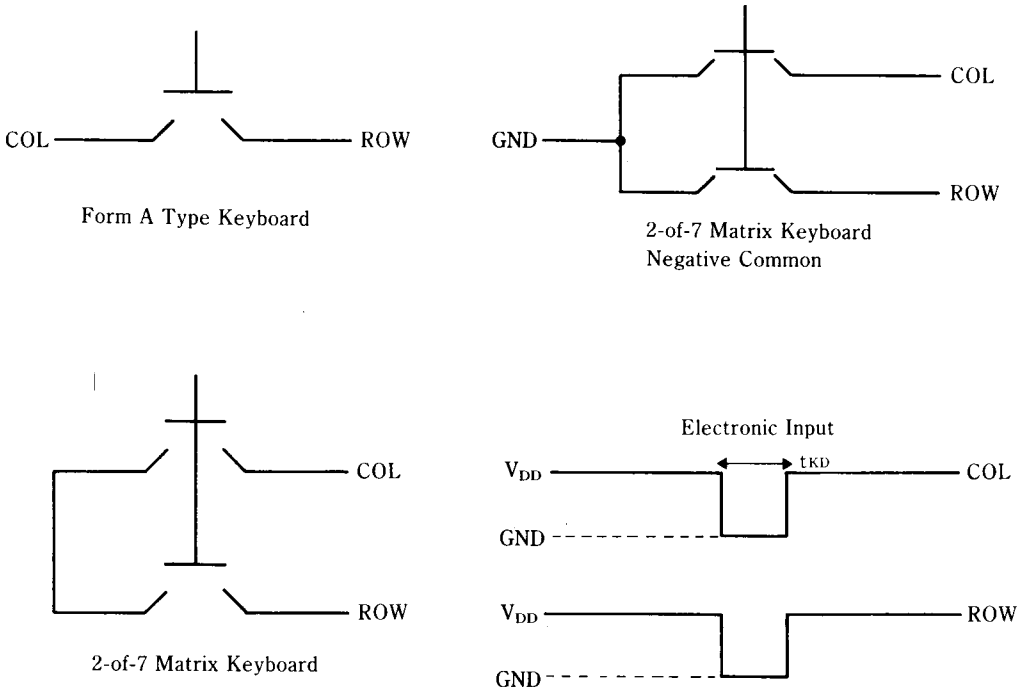
Fig. 2 Keyboard configurations
