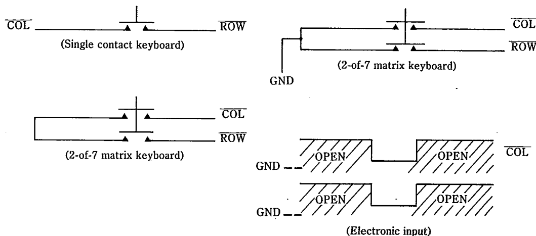
Fig. 1 Keyboard configurations
