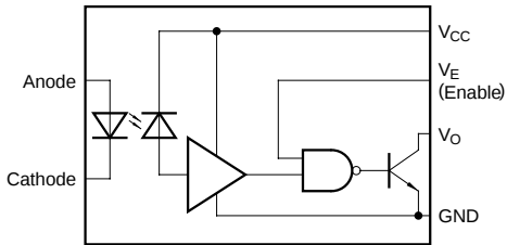
Circuit Block Diagram
