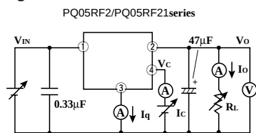
Fig.1 Test Circuit
