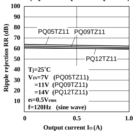
Fig.26 Ripple Rejection vs. Output Current (PQ05TZ11/PQ09TZ11/PQ12TZ11)
