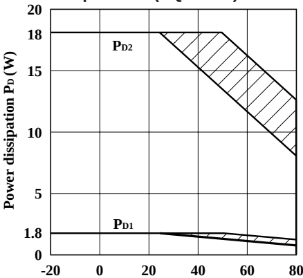
Fig.4 Power dissipation vs. Ambient temperature (PQ3RF33)
