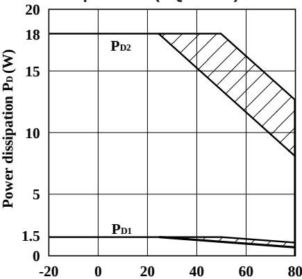
Fig.3 Power Dissipation vs. Ambient Temperature (PQ3RF23)
