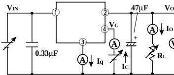
Fig.1 Test Circuit
