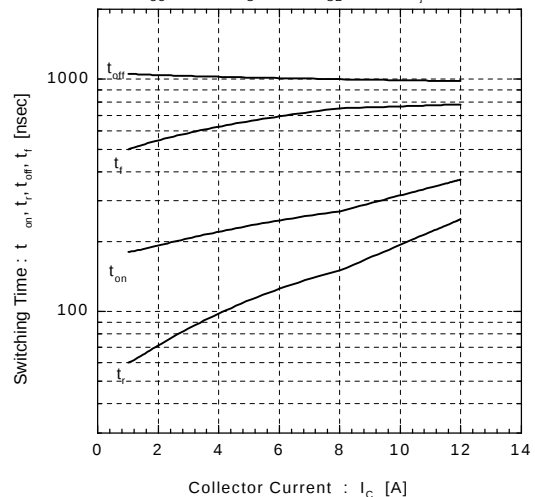
Switching Time vs. Collector Current V_{CC} = 600V, R_G = 20\Omega, V_{GE} = \pm 15V, T_J = 125^\circ\text{C}
