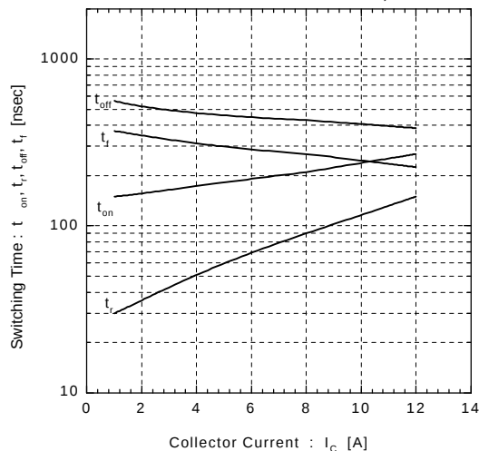
Switching Time vs. Collector Current V_{CC} = 600V, R_G = 20\Omega, V_{GE} = \pm 15V, T_J = 25^\circ\text{C}
