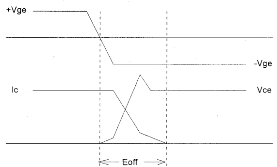
Turn-off Waveforms
