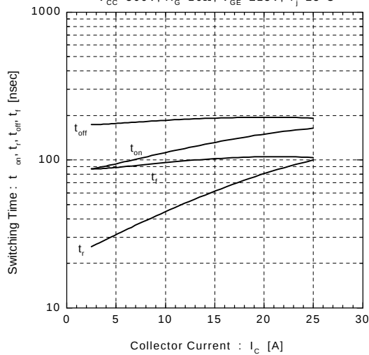
Switching Time vs. Collector Current V_{cc}=300\text{V} , R_g=16\Omega , V_{ge}=\pm 15\text{V} , T_J=25^\circ\text{C}
