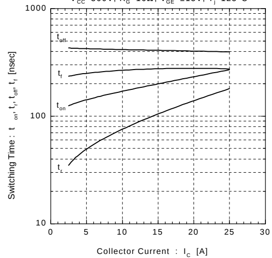
Switching Time vs. Collector Current V_{cc}=300\text{V} , R_g=16\Omega , V_{ge}=\pm 15\text{V} , T_J=125^\circ\text{C}
