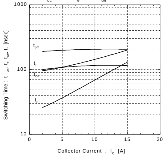
Switching Time vs. Collector Current V_{CC} = 300V, R_G = 22\Omega, V_{GE} = \pm 15V, T_J = 25^\circ\text{C}
