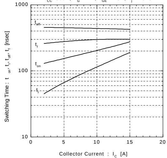
Switching Time vs. Collector Current V_{CC} = 300V, R_G = 22\Omega, V_{GE} = \pm 15V, T_J = 125^\circ\text{C}
