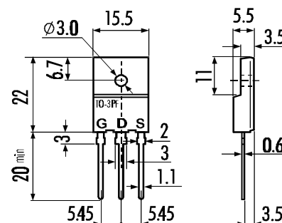
TO-3PF
