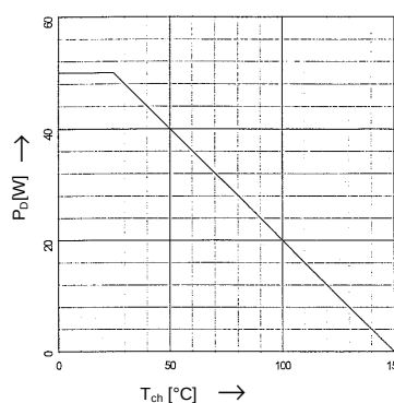
Power Dissipation
