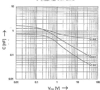
Typical Capacitances
