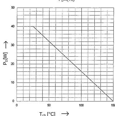
Power Dissipation
