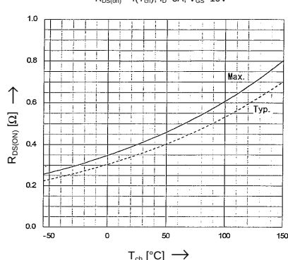
Drain-Source On-State Resistance
