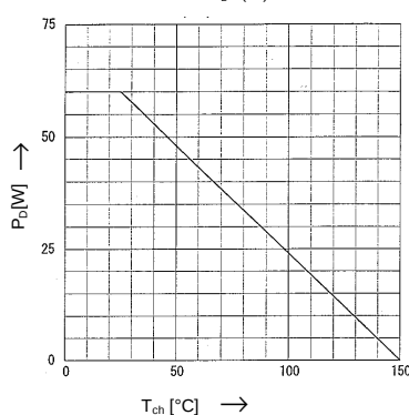
Power Dissipation
