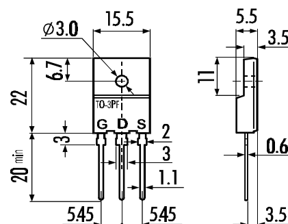
TO-3PF
