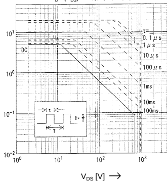
Safe Operation Area
