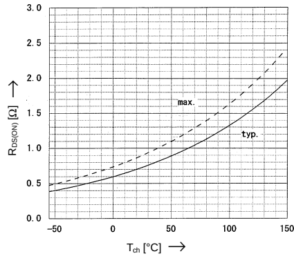
Drain-Source-On-State Resistance vs. T_{ch}
